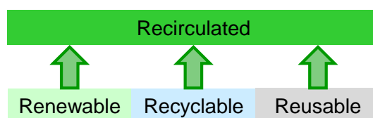
Figure 6: Hierarchy of renewability definitions.
