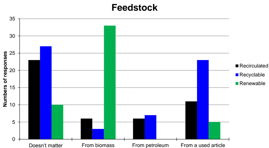
Figure 9: Association of renewability terms with a feedstock.
