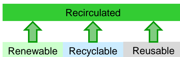
Figure 2: The hierarchy of the renewability definitions.
