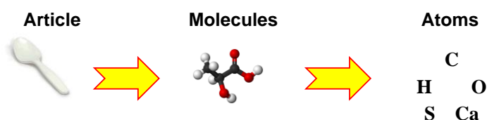
Figure 3: Article, molecules and atoms (e.g. a PLA spoon).
