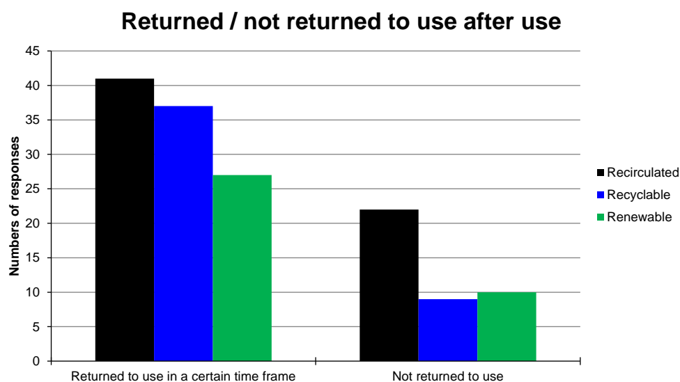
Figure 10: Association of the renewability terms with whether elements are returned to use or not returned to use.
